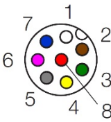
Female connector (at the cable)
