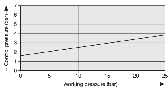
Actuator 43 (DA), flow below the seat
